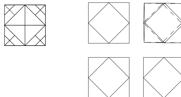
CUBOCTAEDRO
